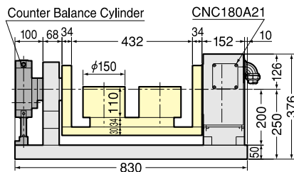
Photo and illustration show the example of the application for un-balancing load.
