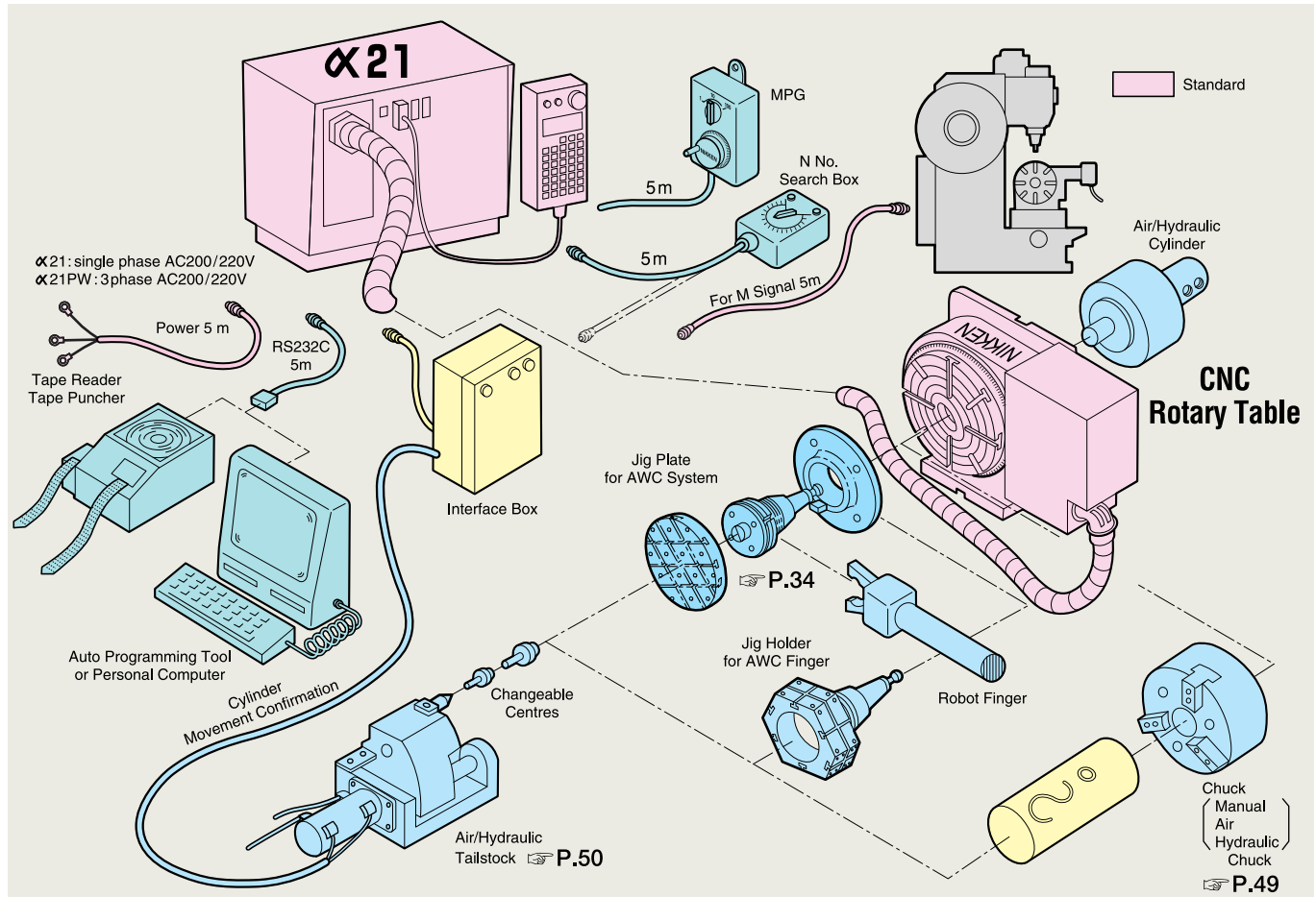
α21 controller for larger capacity (2.7KW, 4.4KW and 11kW) is available. • 3 phase AC200/220V
