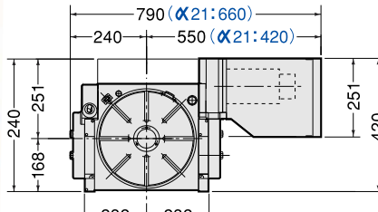
Guide key width: 18mm Table height in horizontal position: 182mm
