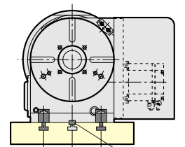
T-slot pitch guide piece
